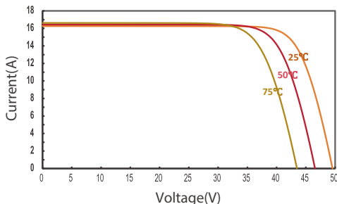
IV Curves of JT635SLt(B) at different Temp.
