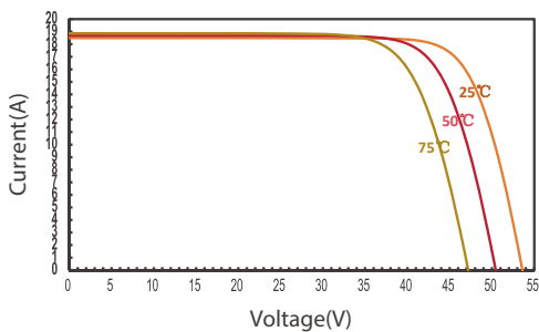
IV Curves of JT780SXt(B) at different Temp.
